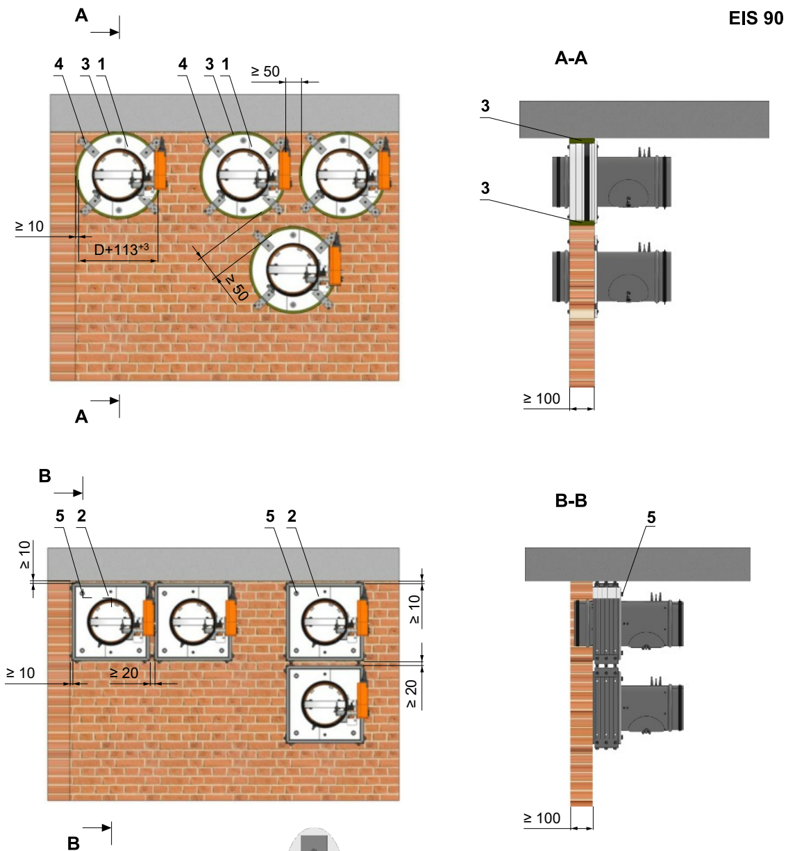
Fitting with steel bracket
