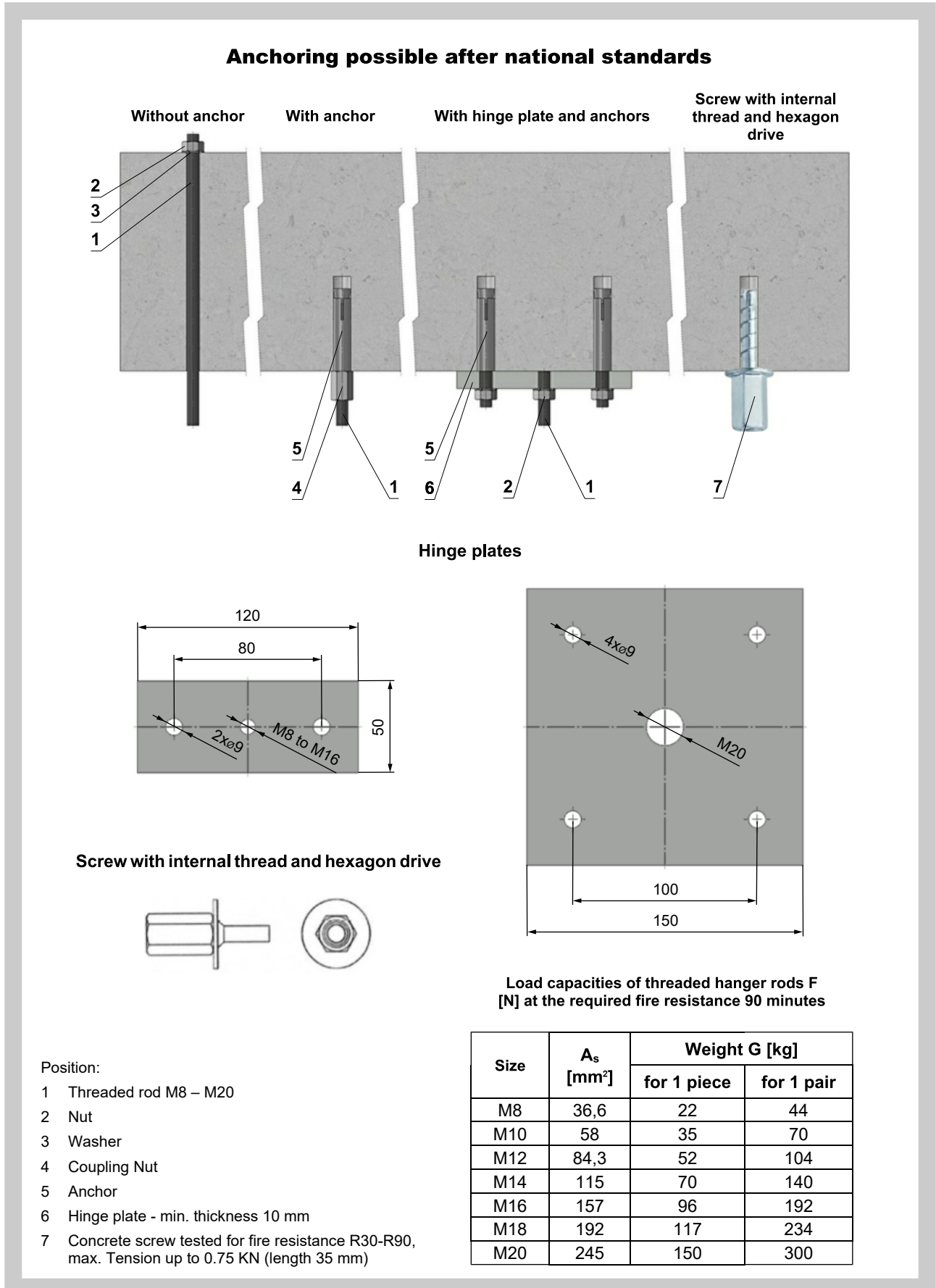
Fig. 95 Mounting to the ceiling wall
