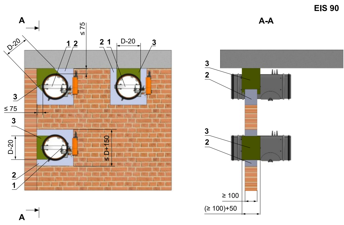
Fig. 42 Solid wall construction - installation next to wall - mortar or gypsum and mineral wool
