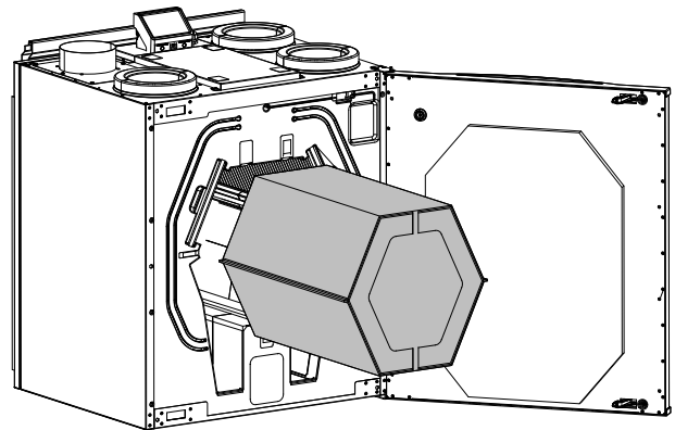
Fig. 4 Heat exchanger
