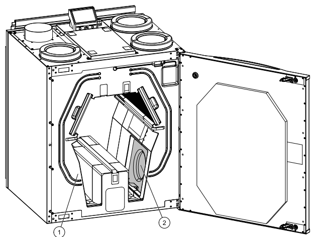
Fig. 5 Supply (pos 1) and extract (pos 2) air fans
